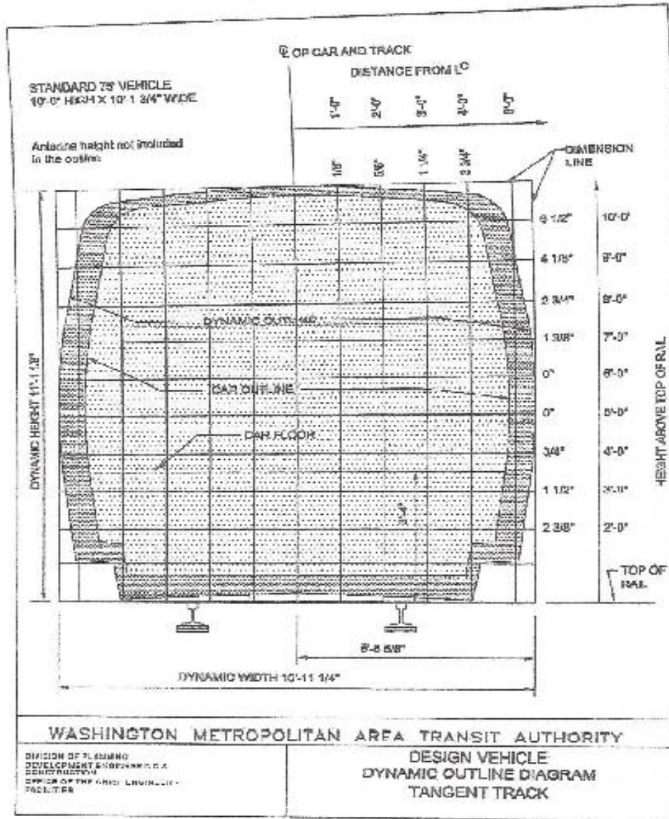
14.1.3 Design Vehicle Dynamic Outline Diagram - Tangent Track
